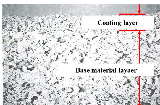
Fig. 5 Cross section of the ceramic filter (microscopic image)
