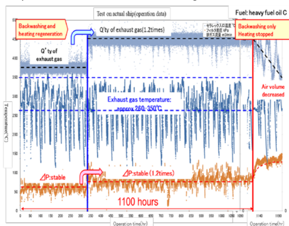
Fig. 9 Changes in differential pressure during prolonged operation
