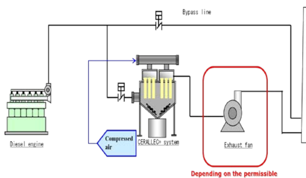
Fig. 7 Diagram of the CERALLEC® system for auxiliary engines
